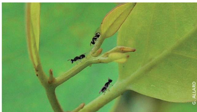
Ovipositing female blue-gum chalcid, Leptocybe invasa
